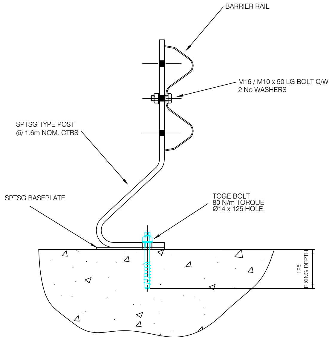
FIXING DETAIL for SPTSG POST with Barrier Rail
